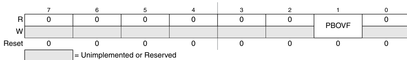
Figure 14-52. Pulse Accumulator B Flag Register (PBFLG)
