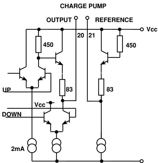
Figure 7f - Charge pump circuit
