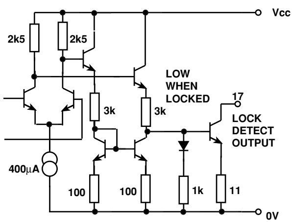
Figure 7d - Lock detect output
