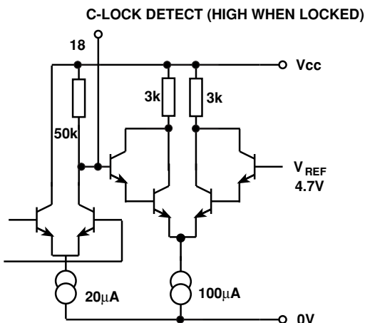
Figure 7c - Lock detect decouple
