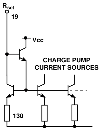
Figure 7e - R set pin
