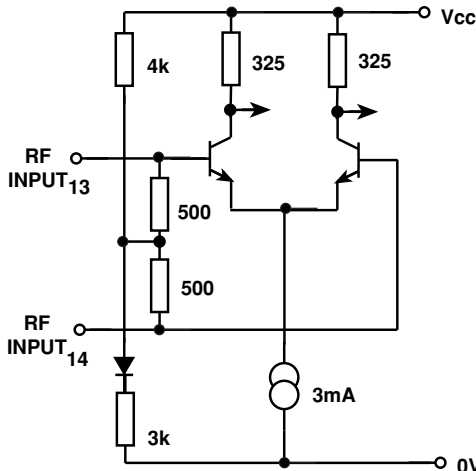
Figure 7b - RF inputs
