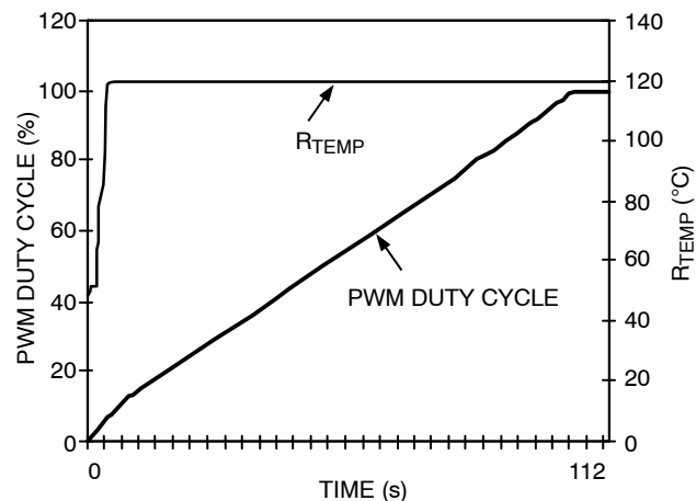
Figure 32. Filtered Mode with Ramp Rate = 1
