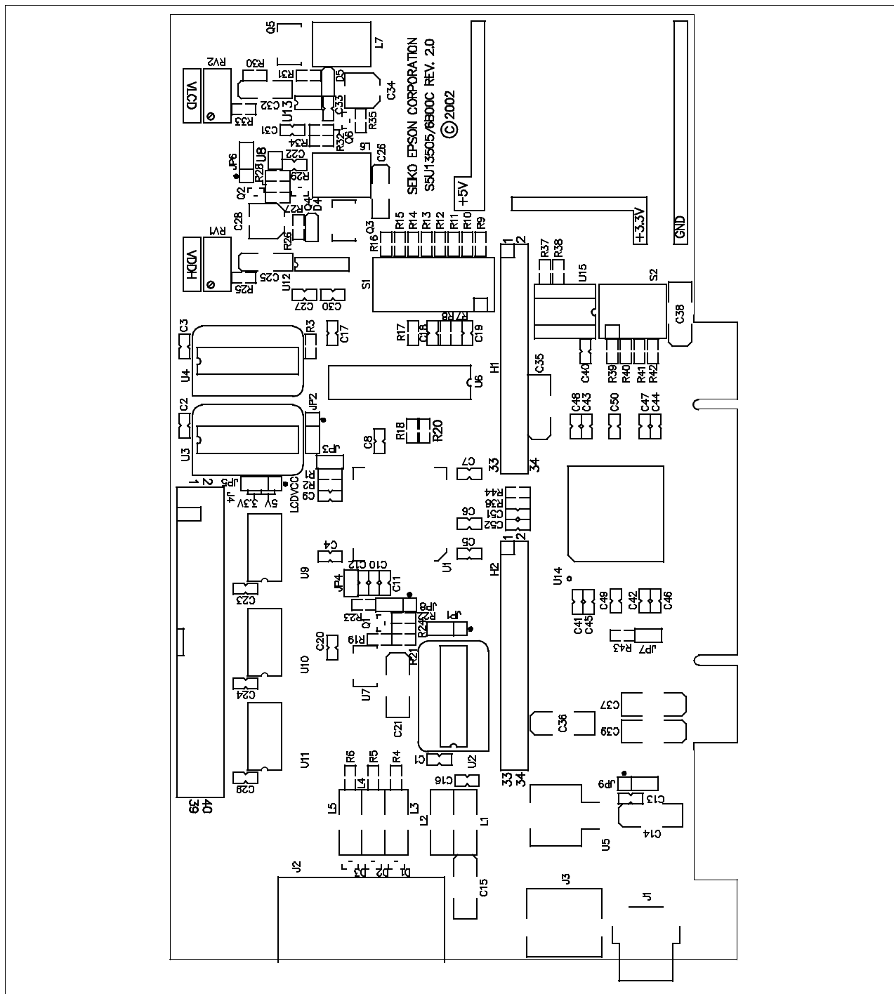
Figure 8-1: S5U13506P00C100 Evaluation Board Layout
