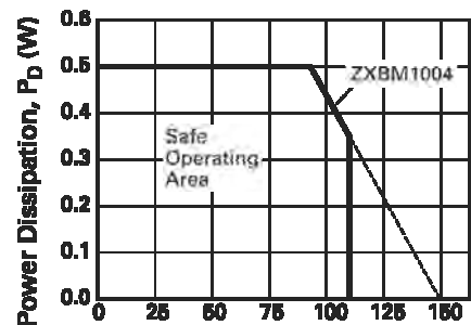
Ambient Temperature, T_A (°C) Power Derating Curve
