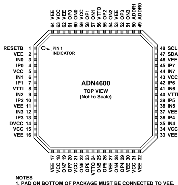
Figure 3. Pin Configuration
