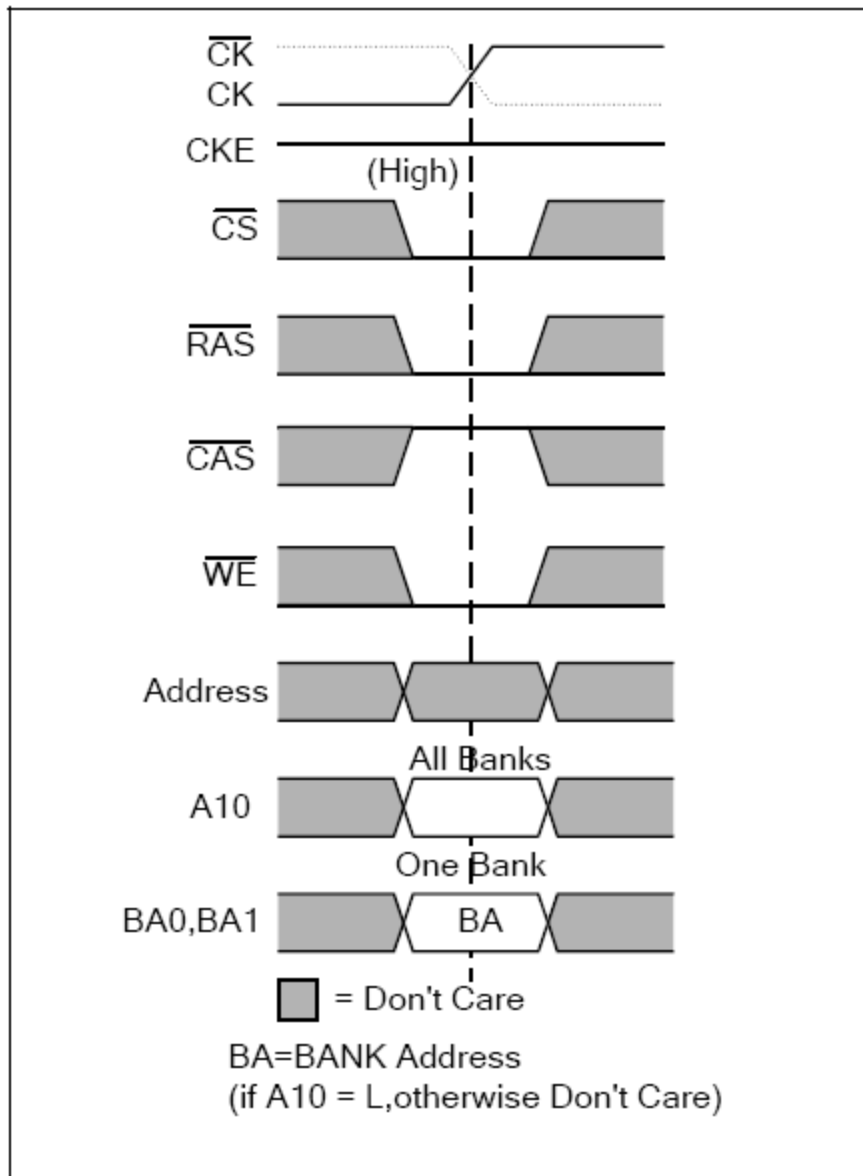
Figure 32 — Precharge command
