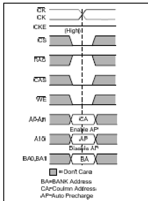
Figure 22 — Write Command
