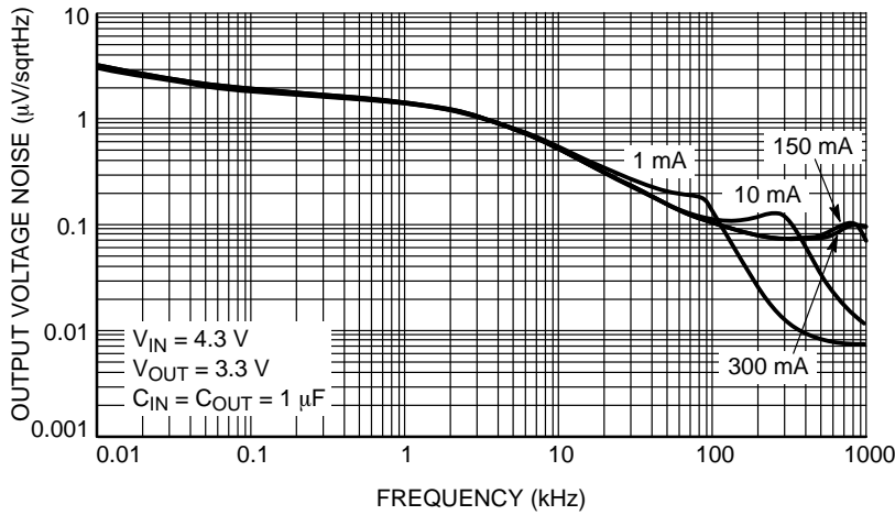
Figure 29. Output Voltage Noise Spectral Density for V_{OUT} = 3.3 V, C_{OUT} = 1 \mu F
