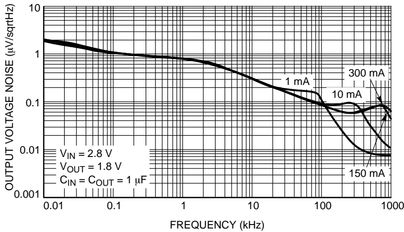
Figure 28. Output Voltage Noise Spectral Density for V_{OUT} = 1.8 V, C_{OUT} = 1 \mu F
