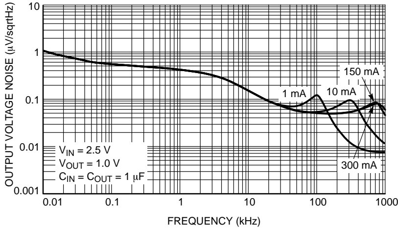
Figure 27. Output Voltage Noise Spectral Density for V_{OUT} = 1.0 V, C_{OUT} = 1 \mu F
