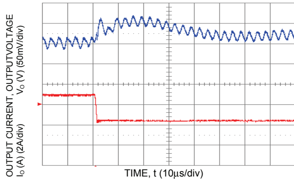
Figure 14. Transient Response to Dynamic Load Change from 100% of 50% full load ( V_o = 5.0\text{ Vdc} , C_{ext} = 2 \times 150\ \mu\text{F} Polymer Capacitors).
