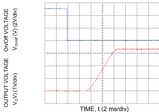
Figure 16. Typical Start-Up Using Remote On/Off with Low-ESR external capacitors ( 7 \times 150\ \mu\text{F} Polymer) ( V_{in} = 5.0\text{ Vdc} , V_o = 3.3\text{ Vdc} , I_o = 5.0\text{ A} , C_o = 1050\ \mu\text{F} ).
