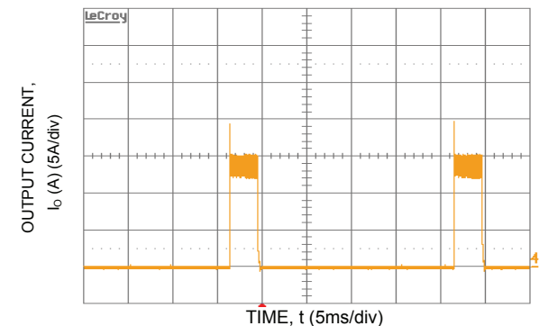
Figure 19. Output short circuit Current ( V_{in} = 5.0\text{ Vdc} , V_o = 0.75\text{ Vdc} ).
