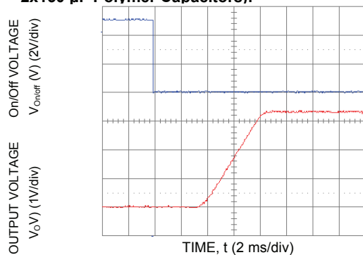
Figure 15. Typical Start-Up Using Remote On/Off ( V_{in} = 5.0\text{ Vdc} , V_o = 3.3\text{ Vdc} , I_o = 5.0\text{ A} ).
