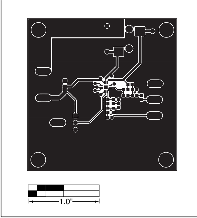
Figure 6. MAX9728A EV Kit PC Board Layout—Component Side
