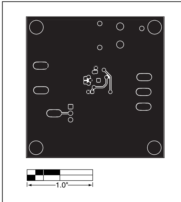
Figure 8. MAX9728A EV Kit PC Board Layout—Solder Side
