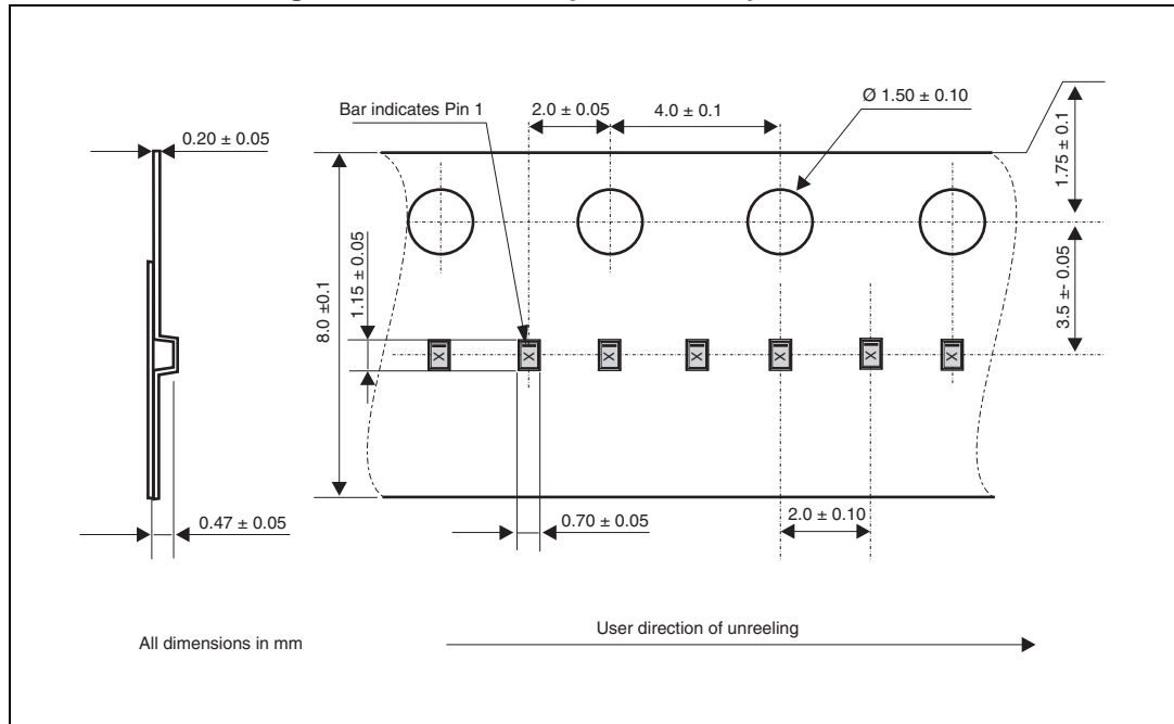
Figure 22. SOD882T tape and reel specifications
