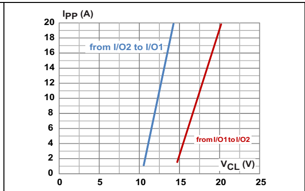
Figure 14. TLP measurement
