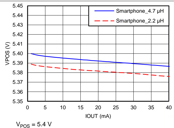
Figure 48. Load Regulation
