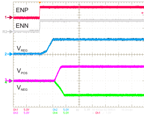
Figure 37. Power-Up Sequencing — Simultaneous
