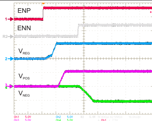
Figure 39. Power-Up Sequencing — Sequential
