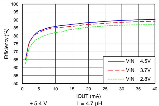
Figure 25. Combined Efficiency — Smartphone
