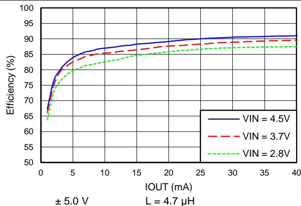
Figure 24. Combined Efficiency — Smartphone
