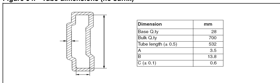
Figure 54. Tube dimensions (no suffix)
