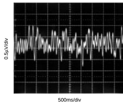
0.1 to 10Hz PEAK-TO-PEAK VOLTAGE NOISE
