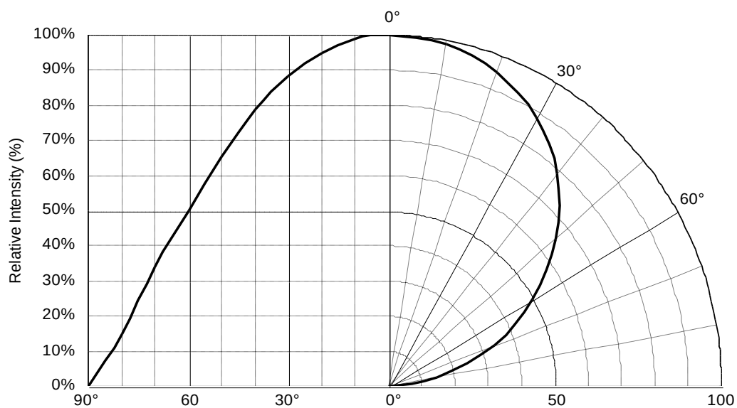
Fig 4. Radiation Characteristics
