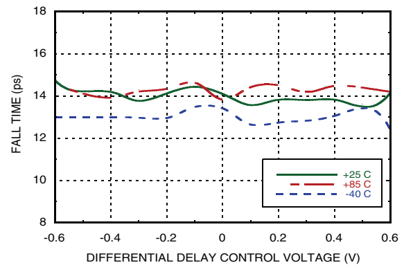
Fall Time vs. Delay Control Voltage [1][2][3][4][6]
