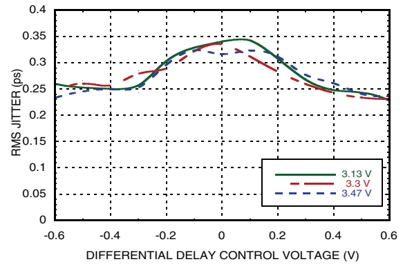
RMS Jitter vs. Delay Control Voltage @ 18GHz [1][2][3][4]
