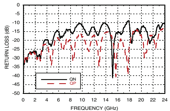
Output Return Loss vs. Frequency [1][2][3]
