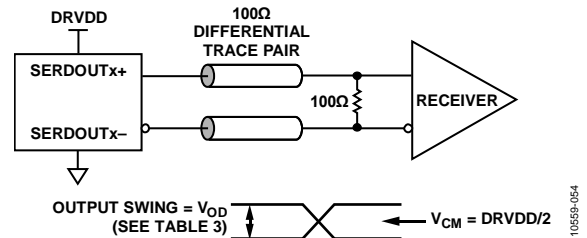
Figure 58. DC-Coupled Digital Output Termination Example
