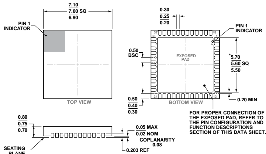
Figure 63. 48-Lead Lead Frame Chip Scale Package [LFCSP_WQ] 7 mm × 7 mm Body, Very Very Thin Quad (CP-48-13)
