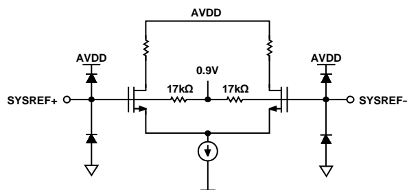
Figure 34. Equivalent SYSREF± Input Circuit
