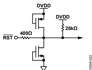
Figure 35. Equivalent \overline{RST} Input Circuit
