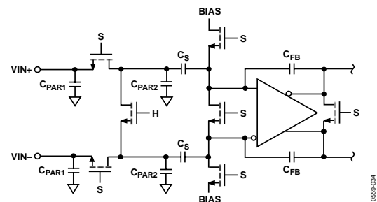
Figure 38. Switched-Capacitor Input
