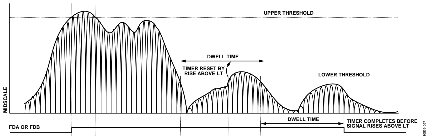
Figure 61. Threshold Settings for FDA and FDB Signals
