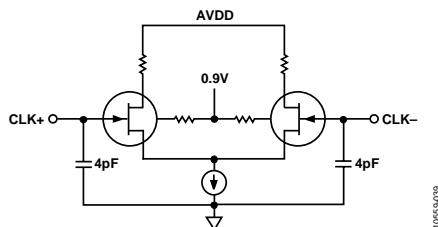
Figure 43. Equivalent Nyquist Clock Input Circuit
