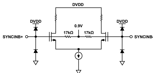
Figure 37. SYNCINB \pm Circuit
