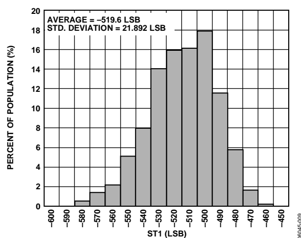
Figure 10. Self-Test 1 Histogram
