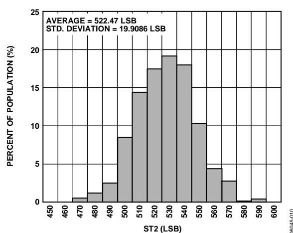
Figure 11. Self-Test 2 Histogram
