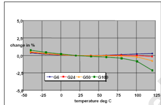
Figure 22: Typical output as function of temperature for all gains
