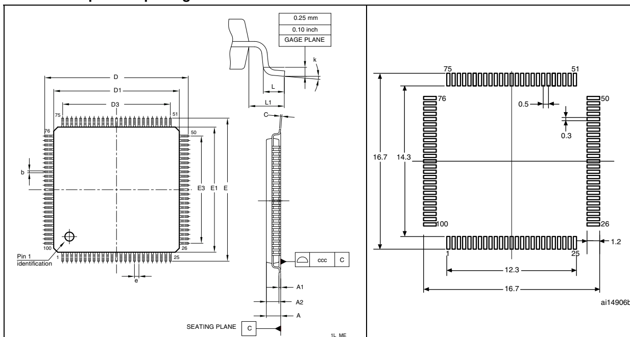
Figure 70. Recommended footprint (1)(2)
