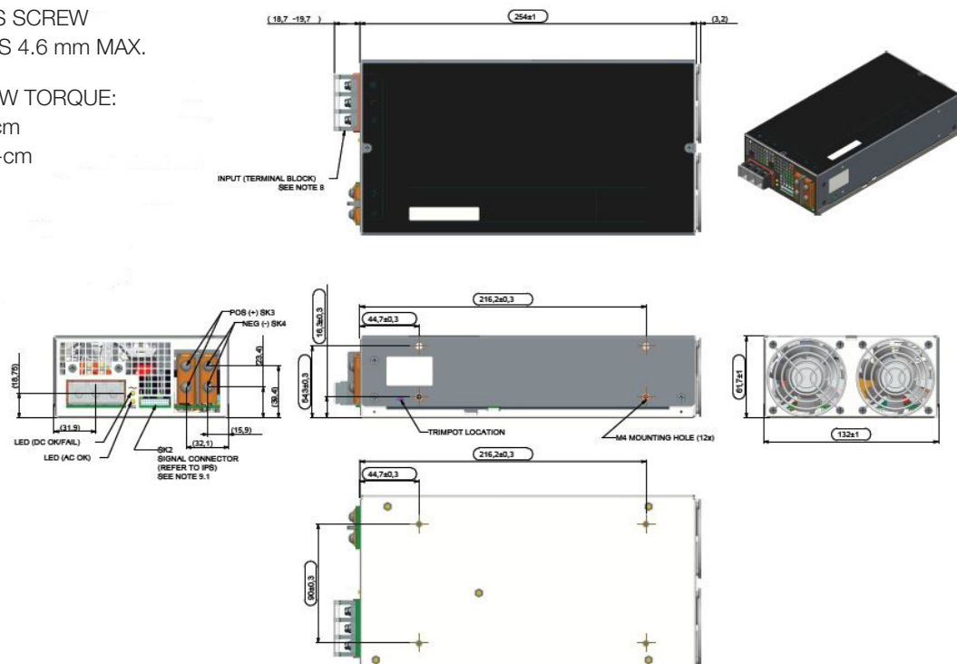
Mechanical Drawings (LCM1500Q-T, LCM1500U-T and LCM1500W-T)
