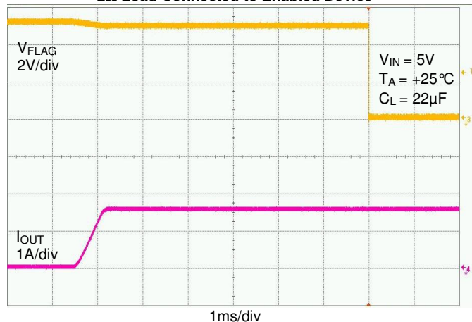
2Ω Load Connected to Enabled Device
