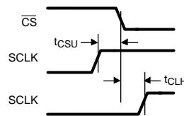
Figure 6. SCLK and CS Timing Parameters
