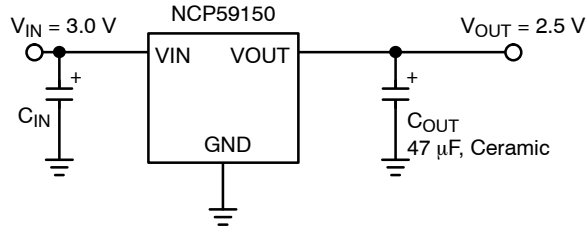
Figure 3. Fixed 2.5 Regulator in D²PAK-3 Package
