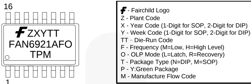
Figure 3. Marking Diagram
