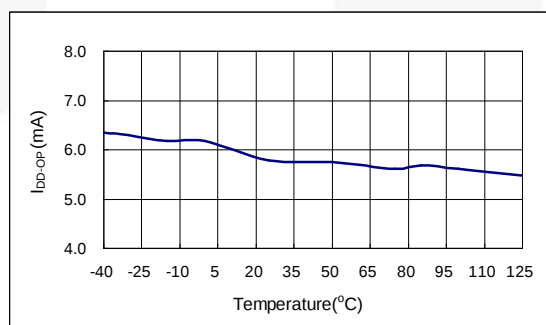
Figure 10. Operating Current
