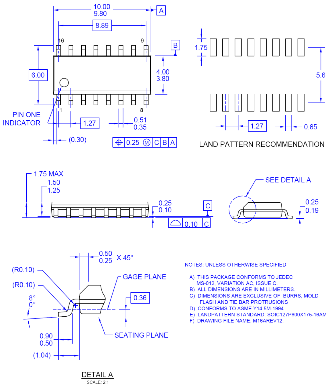
Figure 46. 16-Pin Small Outline Package (SOP)
