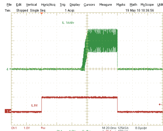
Figure 5. Charge Enable by ILIM
