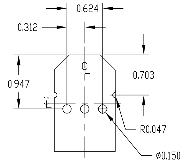
PC BOARD LAYOUT OPTION #2
