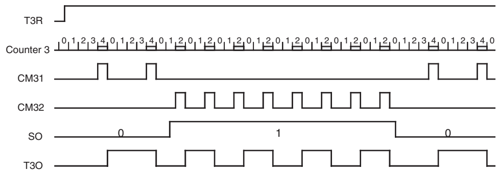
Figure 24-18. FSK Modulation
