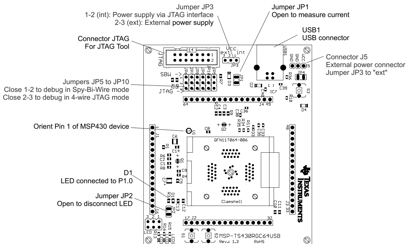
Figure B-46. MSP-TS430RGC64USB Target Socket Module, PCB
