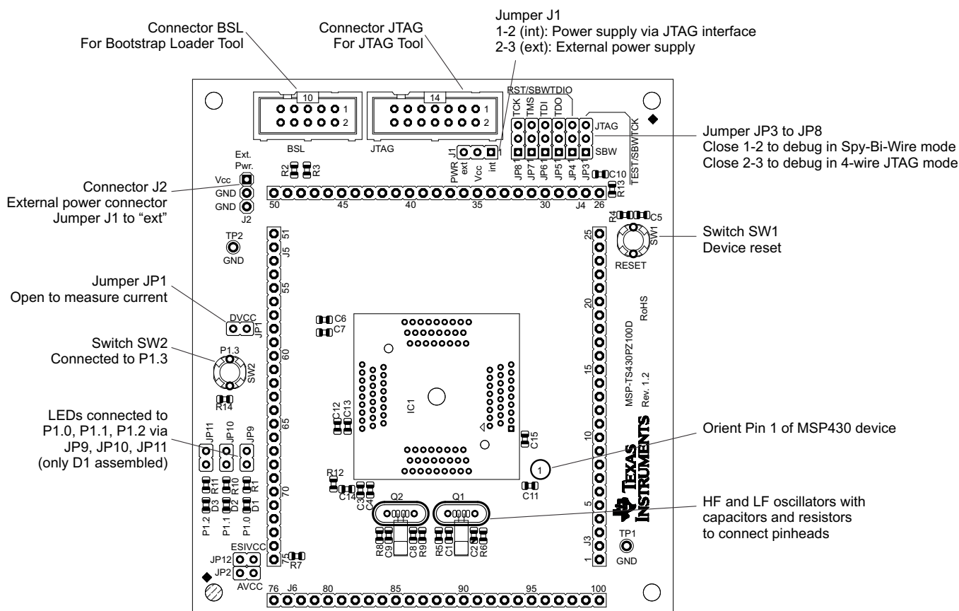
Figure B-62. MSP-TS430PZ100D Target Socket Module, PCB
