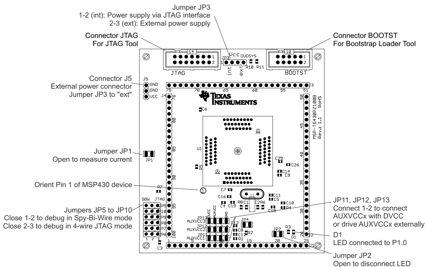
Figure B-58. MSP-TS430PZ100B Target Socket Module, PCB
