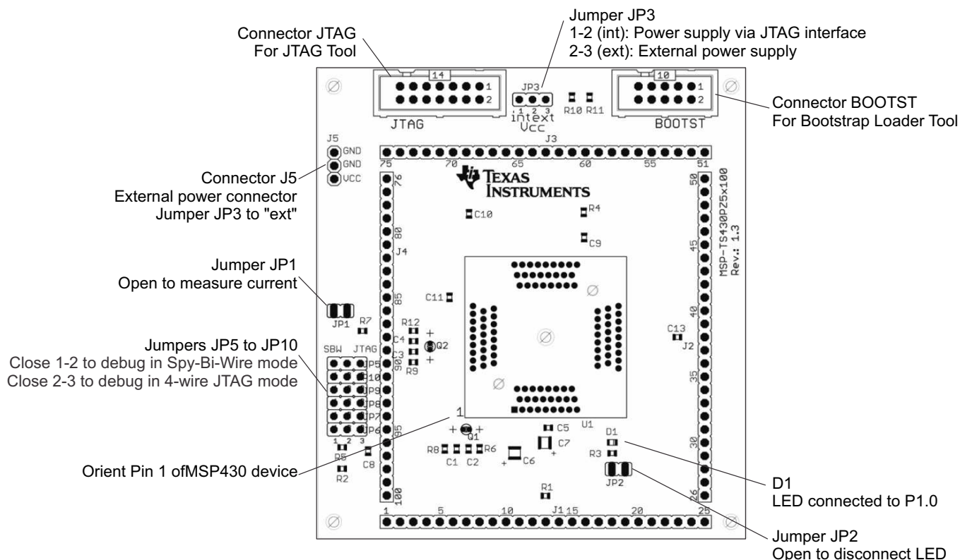
Figure B-64. MSP-TS430PZ5x100 Target Socket Module, PCB
