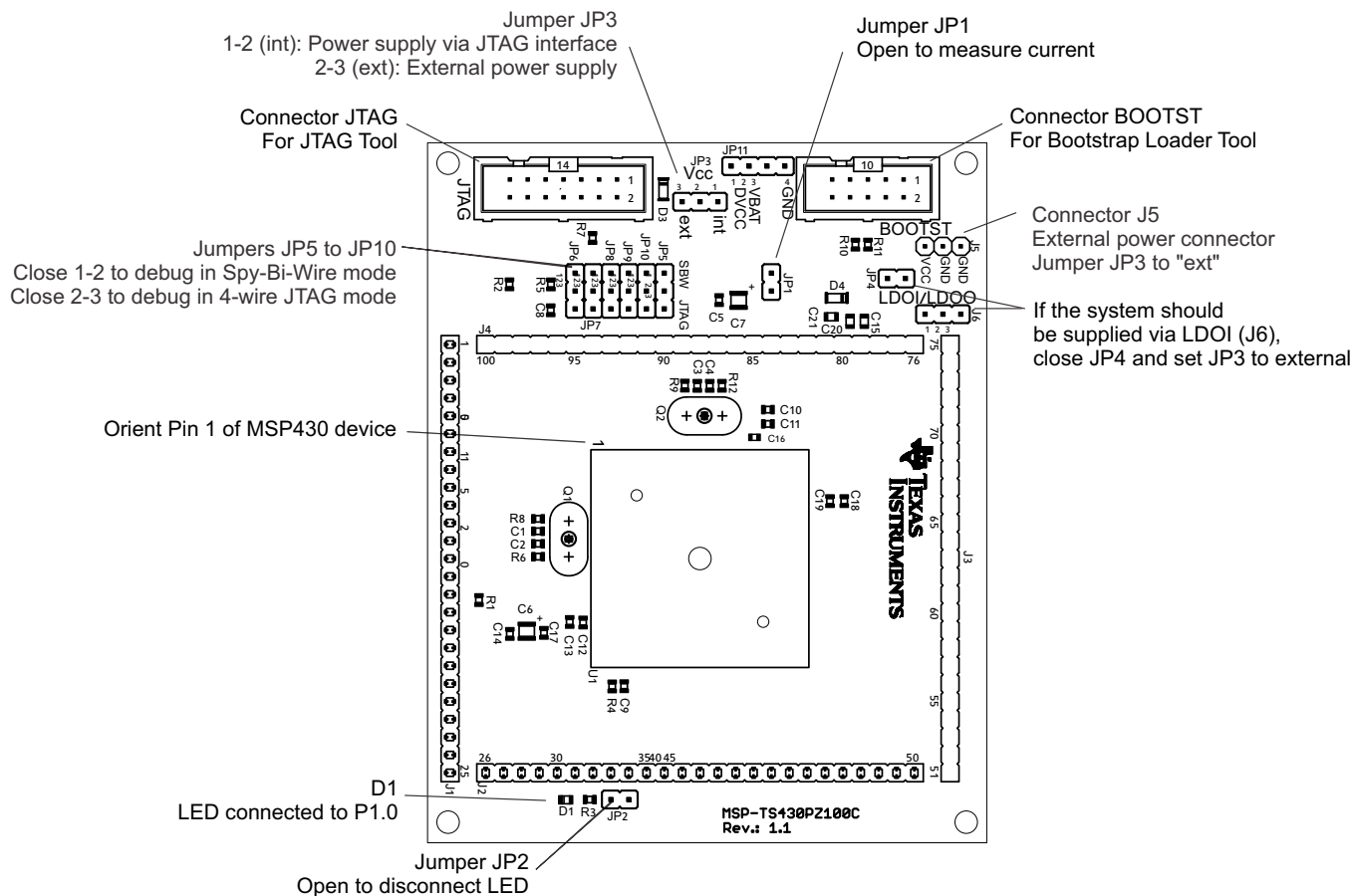
Figure B-60. MSP-TS430PZ100C Target Socket Module, PCB
