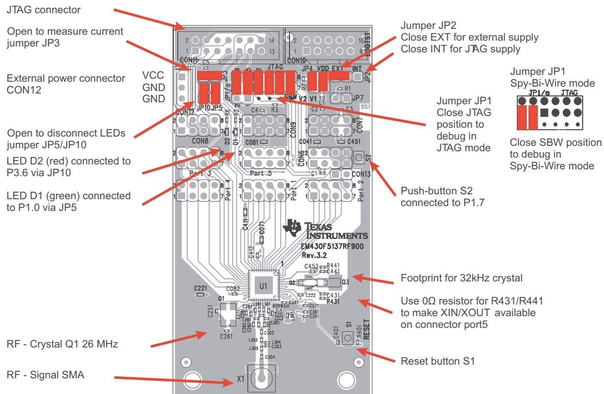
Figure B-72. EM430F5137RF900 Target board, PCB
