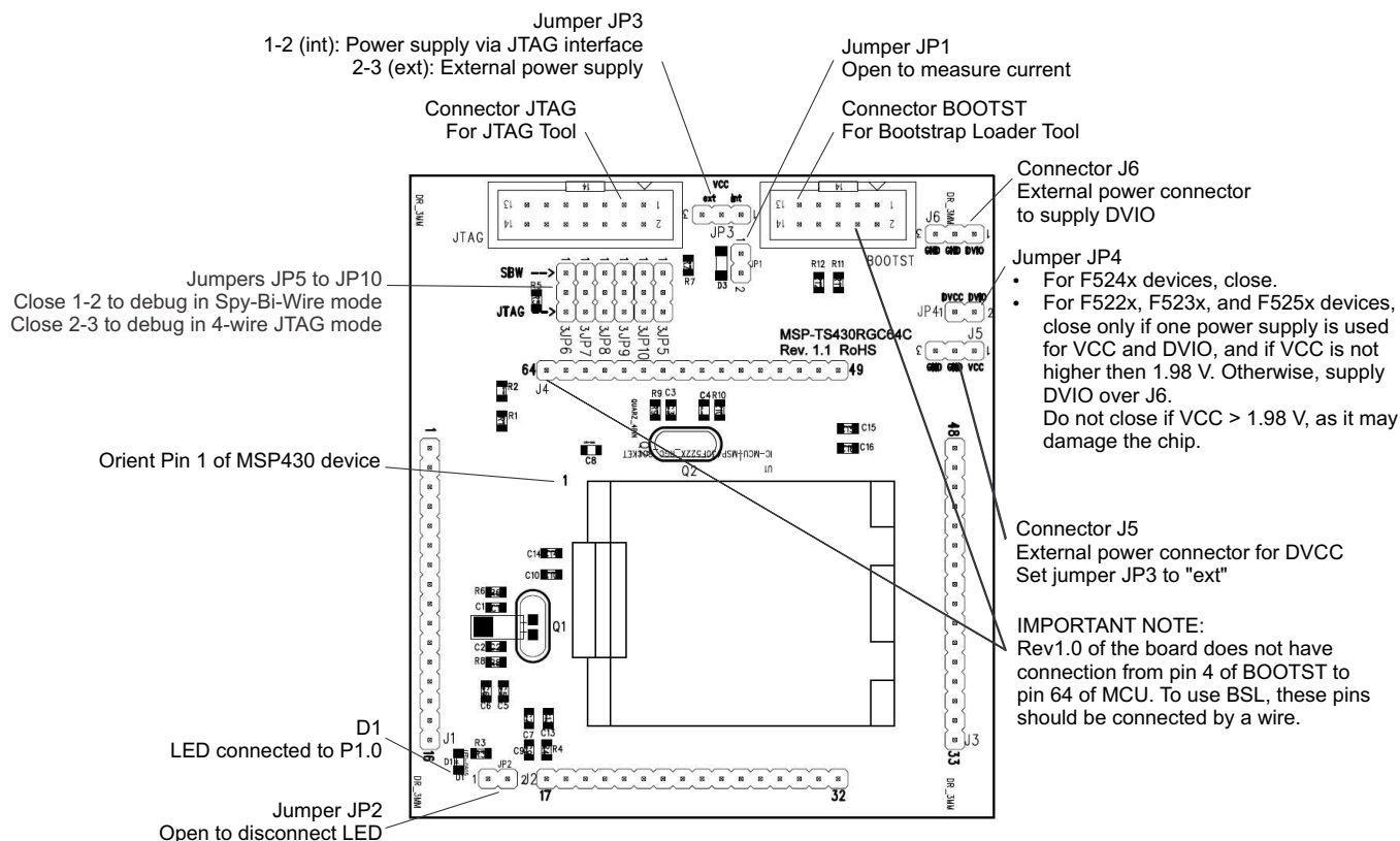
Figure B-44. MSP-TS430RGC64C Target Socket Module, PCB
