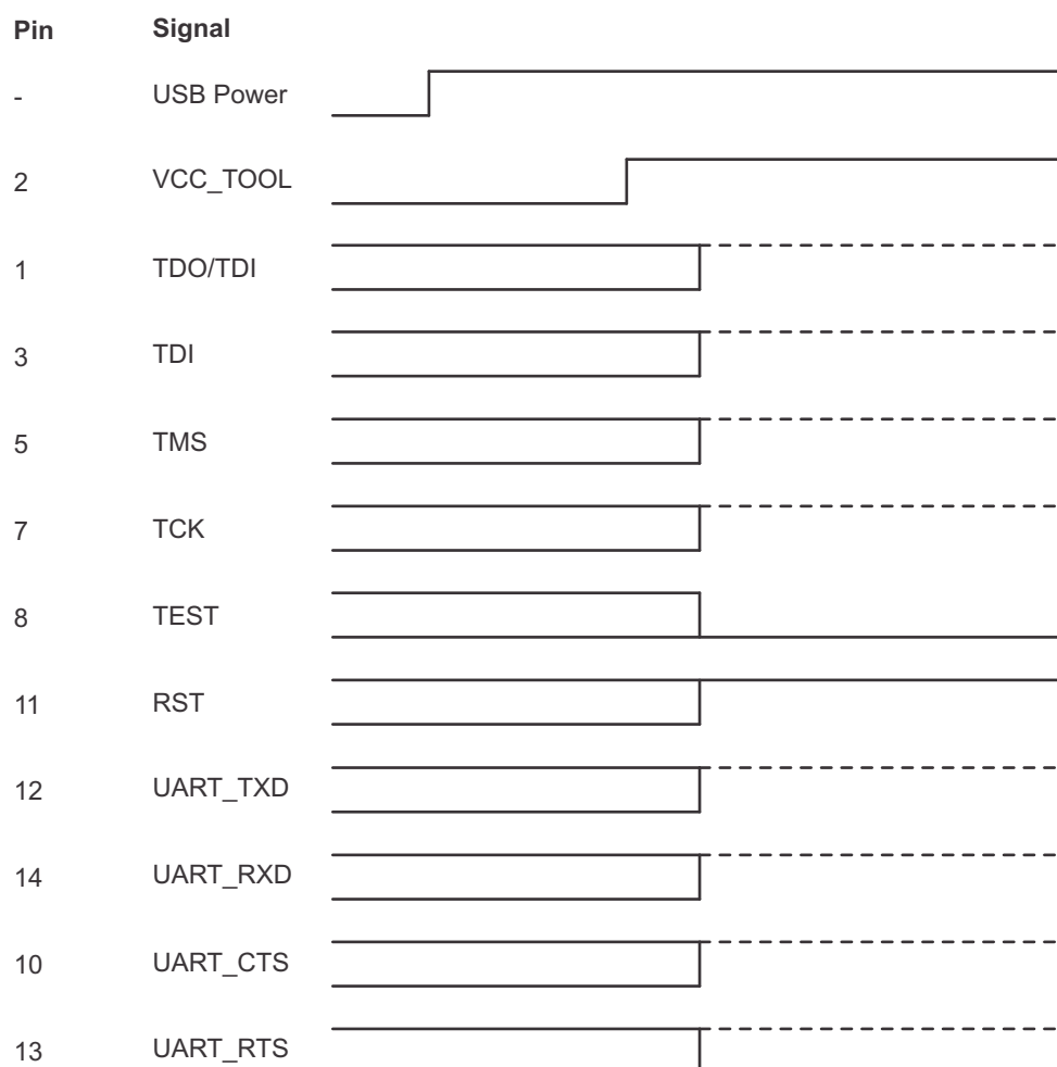
Figure B-87. Pin States After Power-Up
