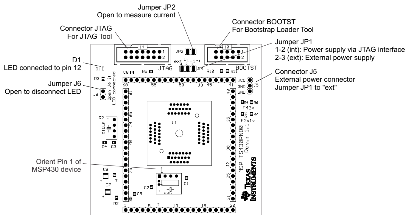
Figure B-48. MSP-TS430PN80 Target Socket Module, PCB
