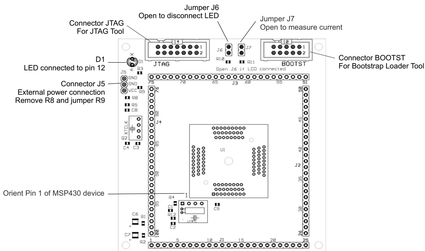
Figure B-54. MSP-TS430PZ100 Target Socket Module, PCB
