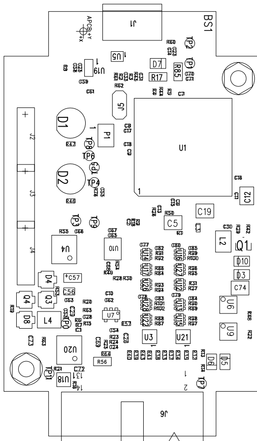
Figure B-84. MSP-FET USB Debugger, PCB (Top)
