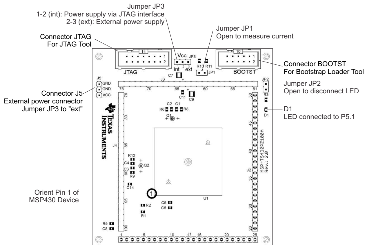
Figure B-56. MSP-TS430PZ100A Target Socket Module, PCB
