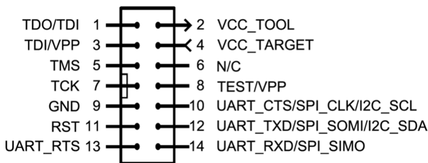
Figure B-86. JTAG Connector Pinout
