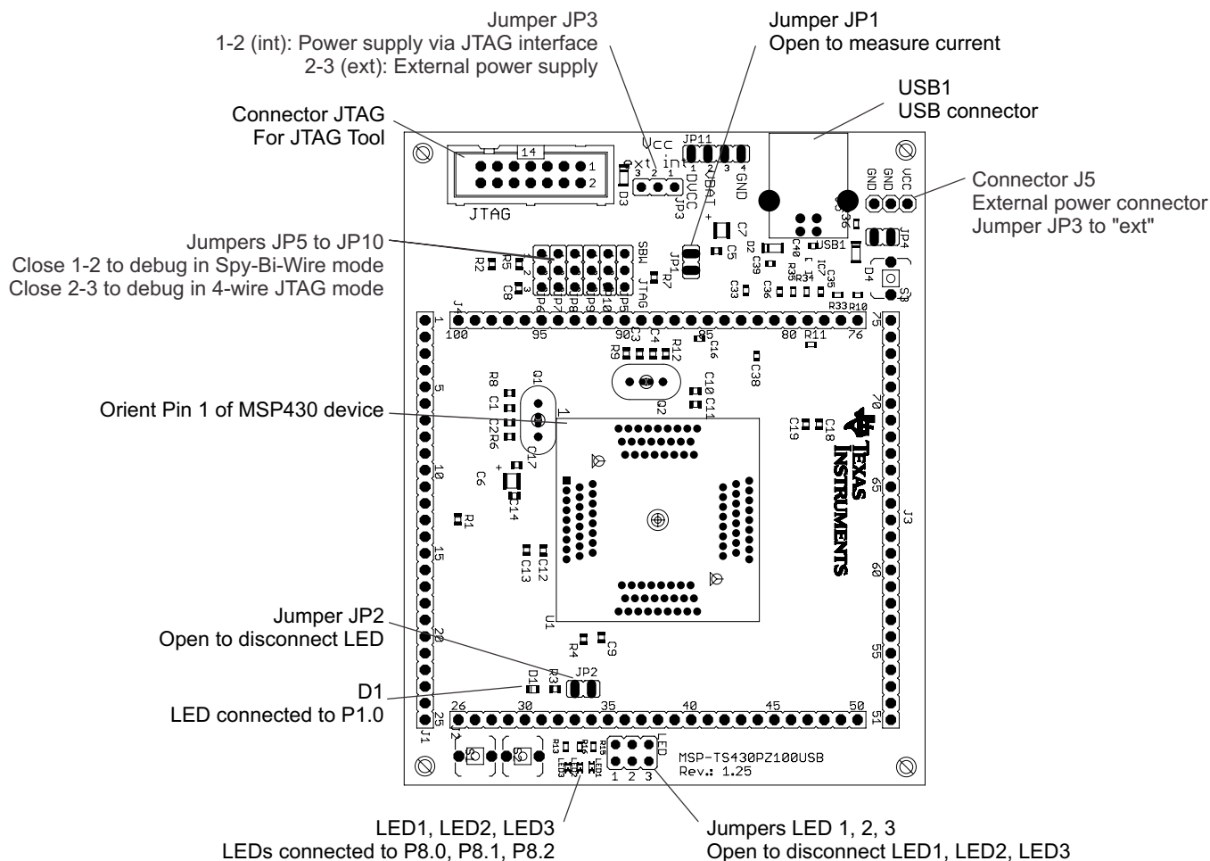
Figure B-66. MSP-TS430PZ100USB Target Socket Module, PCB
