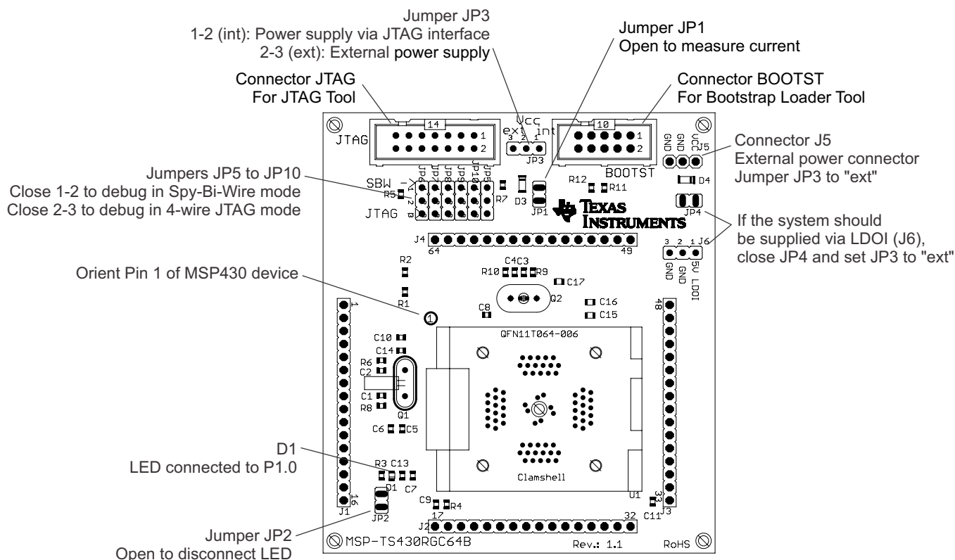
Figure B-42. MSP-TS430RGC64B Target Socket Module, PCB
