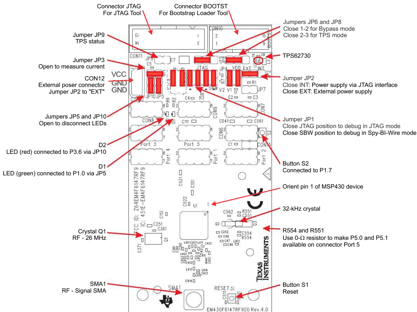
Figure B-76. EM430F6147RF900 Target Board, PCB
