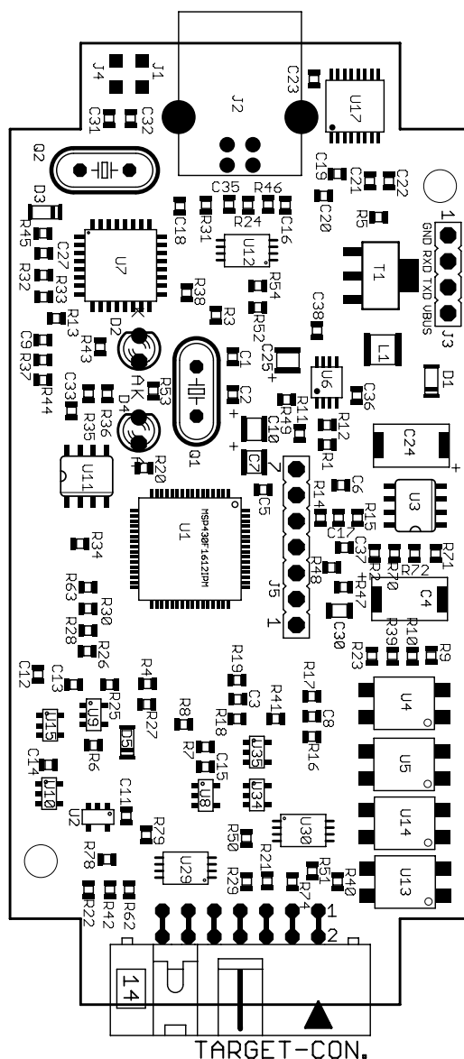
Figure B-94. MSP-FET430UIF USB Interface, PCB
