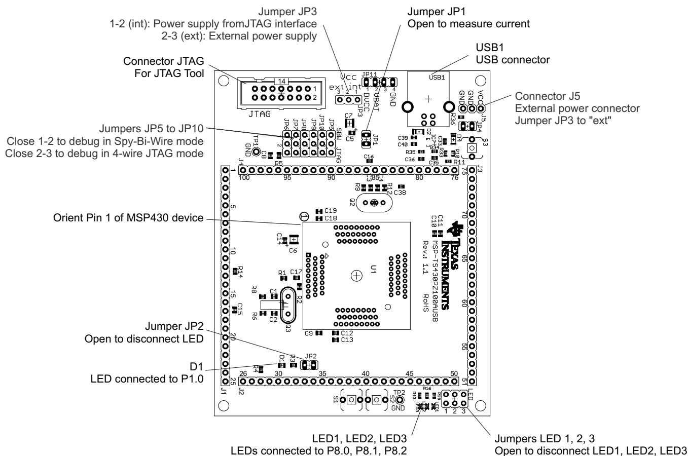
Figure B-68. MSP-TS430PZ100AUSB Target Socket Module, PCB
