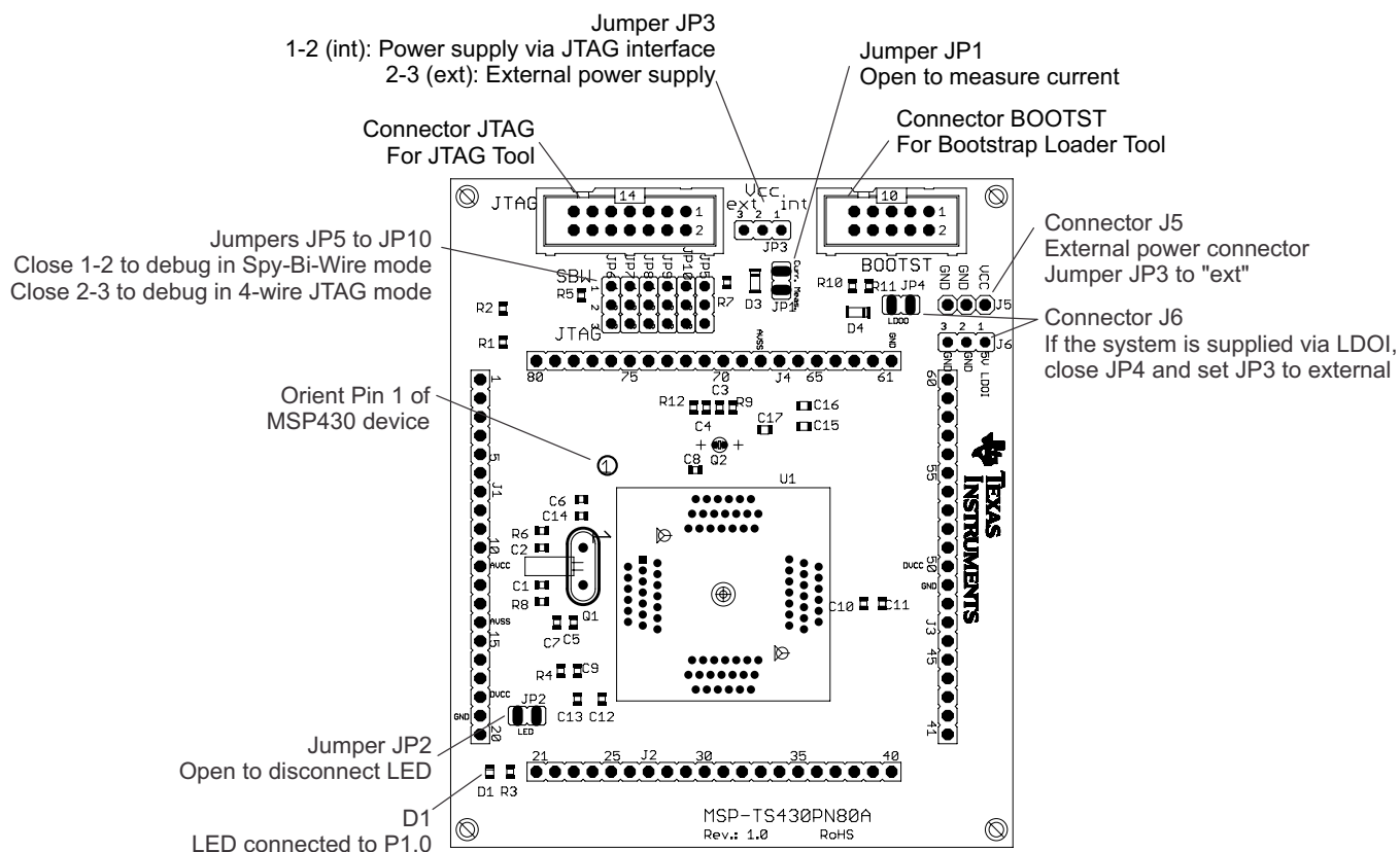
Figure B-50. MSP-TS430PN80A Target Socket Module, PCB
