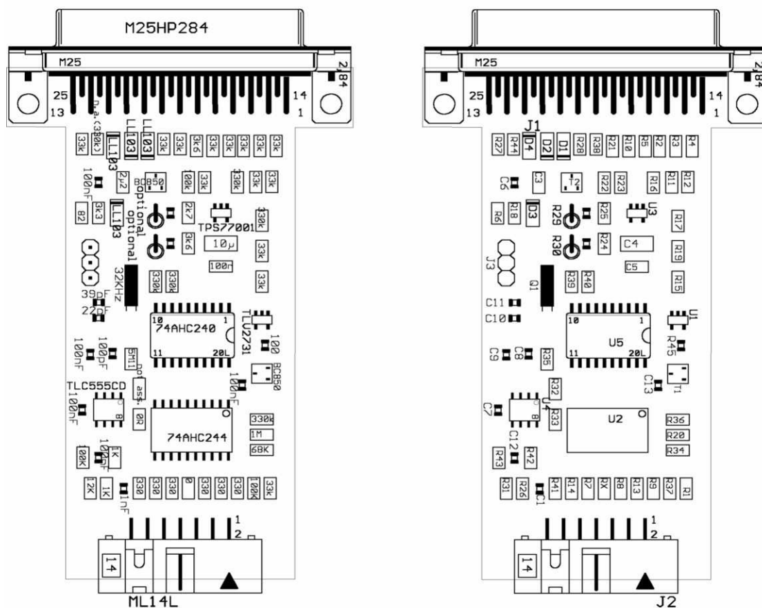
Figure B-89. MSP-FET430PIF FET Interface Module, PCB
