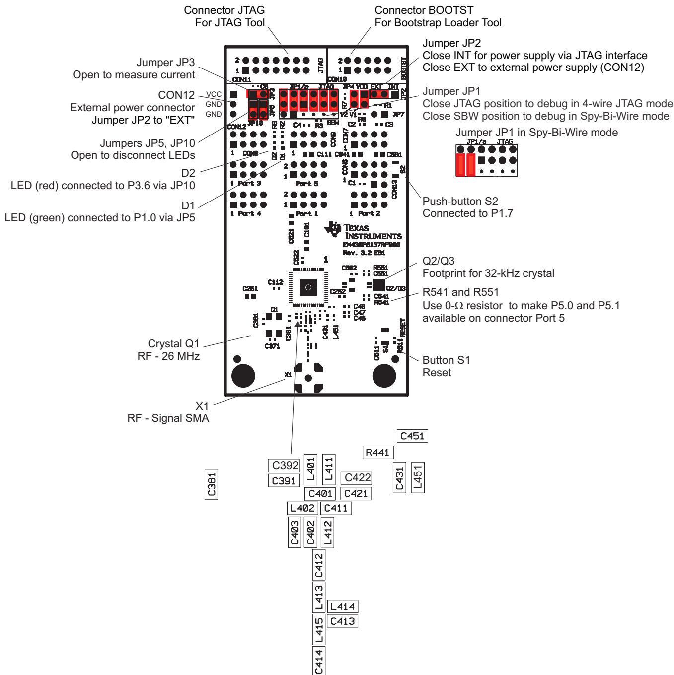
Figure B-74. EM430F6137RF900 Target Board, PCB
