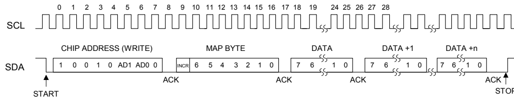
Figure 23. Control Port Timing, I²C Write
