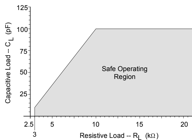
Figure 3. Maximum Loading
