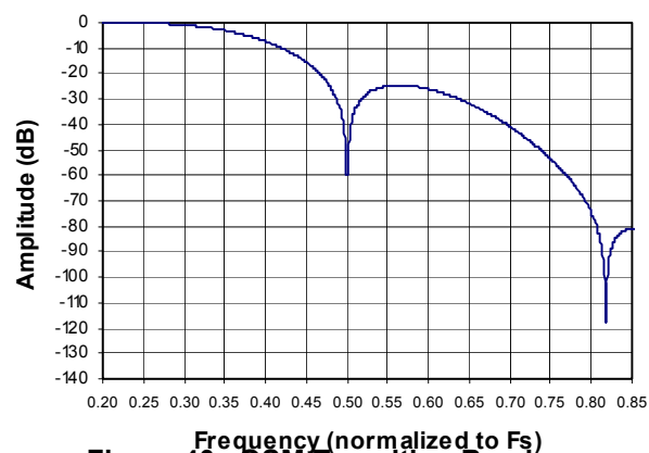
Figure 40. QSM Transition Band
