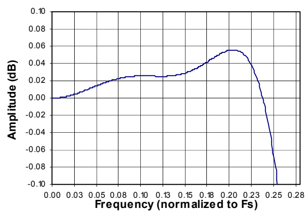
Figure 42. QSM Passband Ripple
