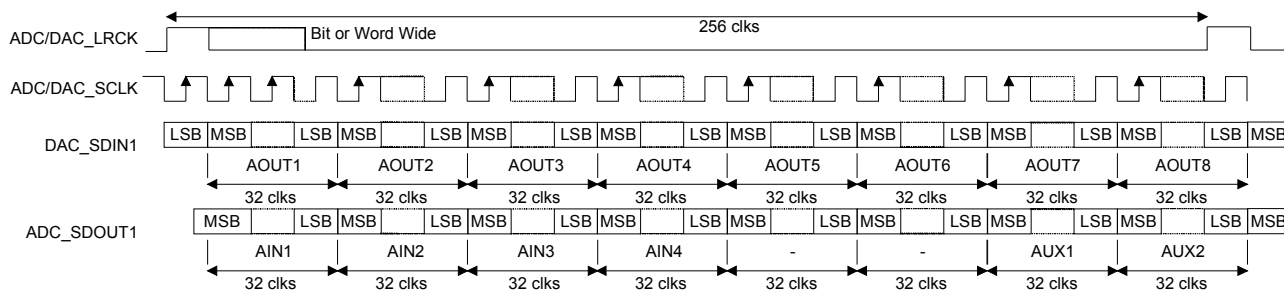
Figure 19. TDM Format
