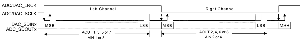
Figure 15. Left-Justified Format
