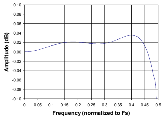
Figure 34. SSM Passband Ripple
