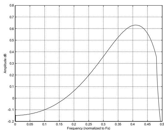
Figure 50. DSM Passband Ripple
