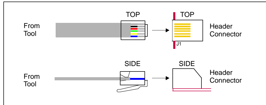
FIGURE 1: MODULAR CONNECTION
