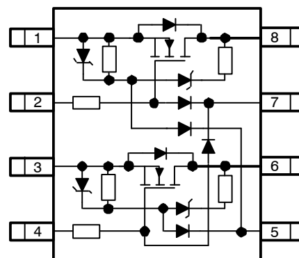
INTERNAL DIAGRAM
