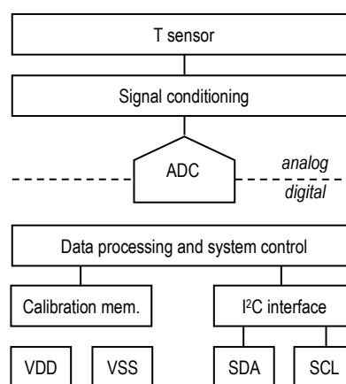
Figure 1 Functional block diagram of the STSC1.
