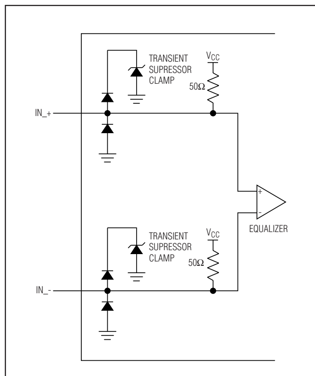
Figure 2. Simplified Input Circuit
