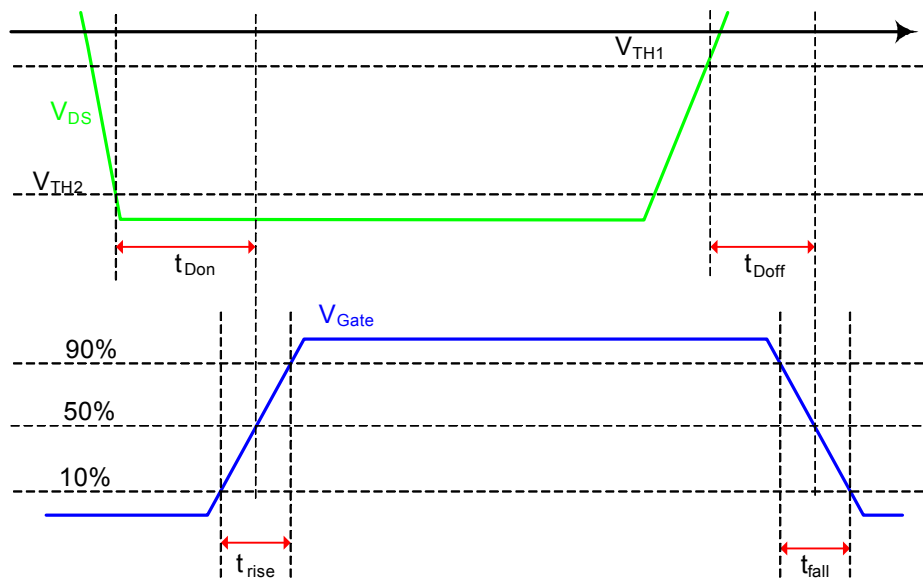
Fig. 15 - Timing Diagrams
