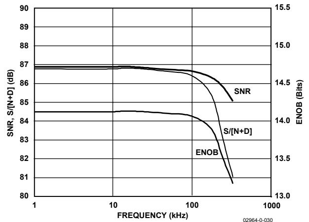
Figure 10. SNR, \text{S}/[\text{N}+\text{D}] , and ENOB vs. Frequency
