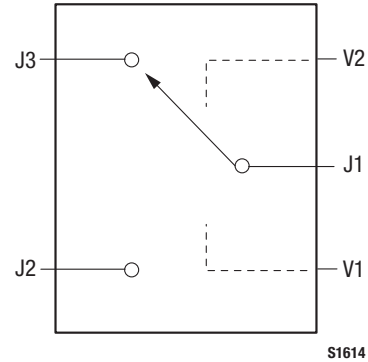
Figure 1. AS179-92LF Block Diagram
