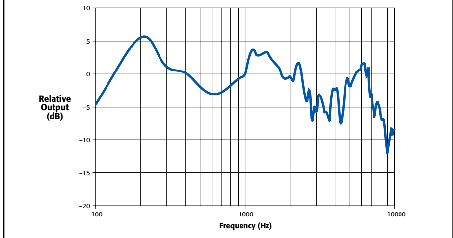
Figure 4. Frequency Response
