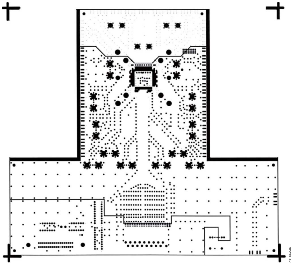
Figure 49. INT1 ( V_{EE} )
