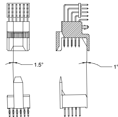
INCLINATION TOLERANCES
