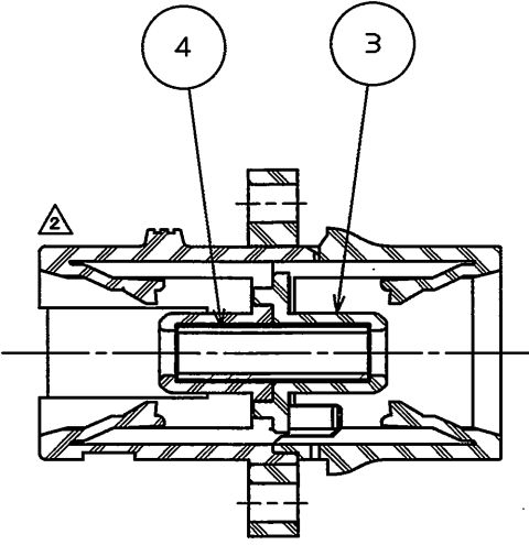
SECT. A-A
