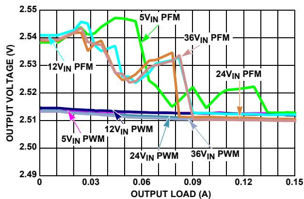
FIGURE 15. V_{OUT} REGULATION vs LOAD, V_{OUT} = 2.5\text{V}
