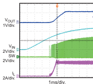
V_{IN} Power Up with 3A Load
