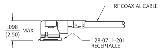
MP Plug (Medium Profile Plug)
