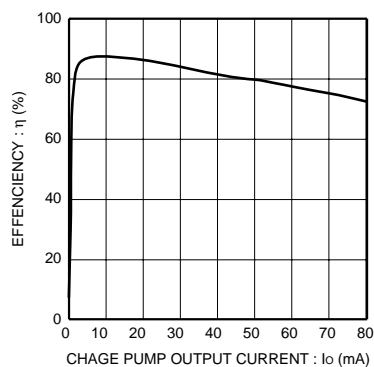
Fig.5 Effenciency-load current (note1)
