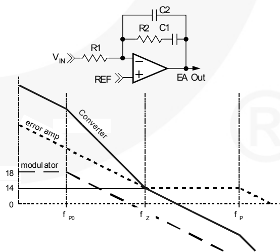
Figure 14. Compensation
