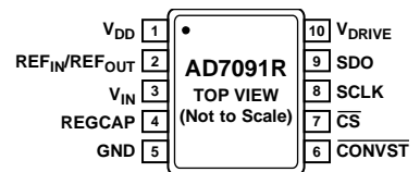
Figure 4. Pin Configuration, 10-Lead MSOP
