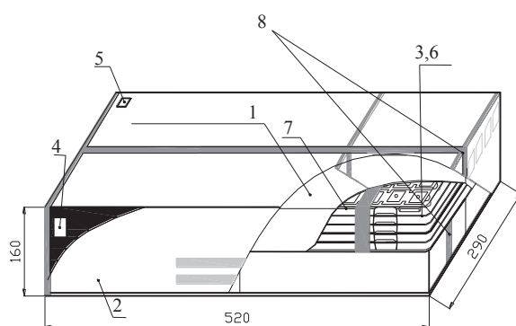
Inner Box dimensions (unit: mm)
