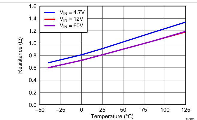
Figure 2. Low-Side R_{DS(on)} vs Temperature
