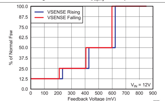
Figure 4. Frequency vs V_{SENSE} Voltage
