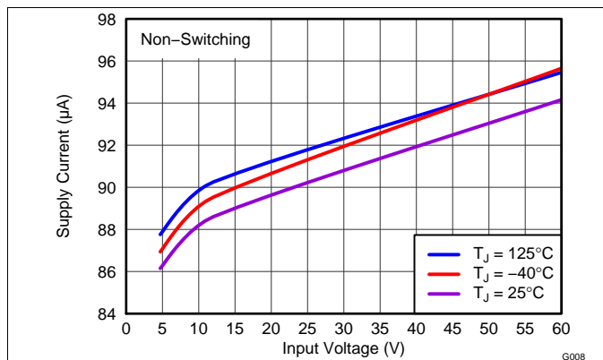
Figure 13. Supply Current (VIN pin) vs Input Voltage
