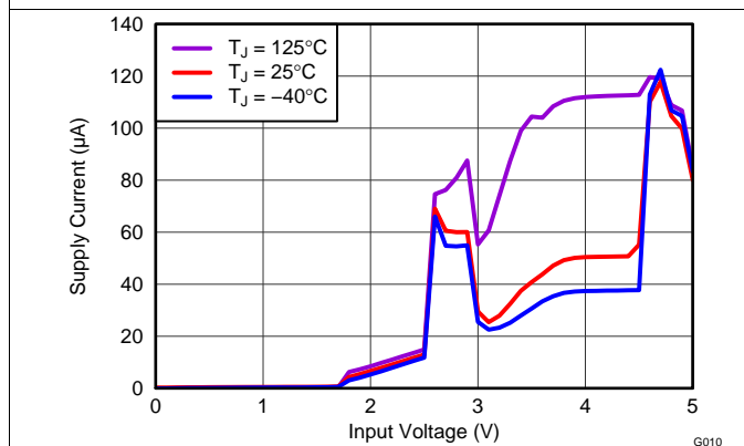
Figure 15. Supply Current (VIN pin) vs Input Voltage (0V to VSTART) EN Pin Open
