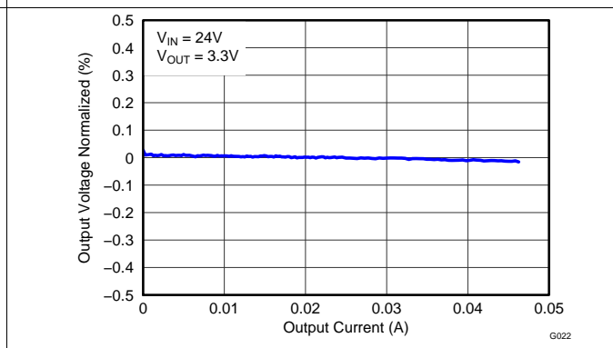
Figure 40. Output Voltage vs Output Current
