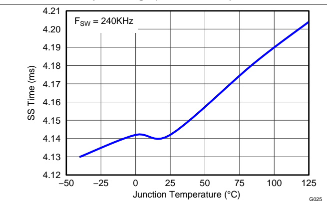
Figure 16. Slow-Start Time vs Temperature
