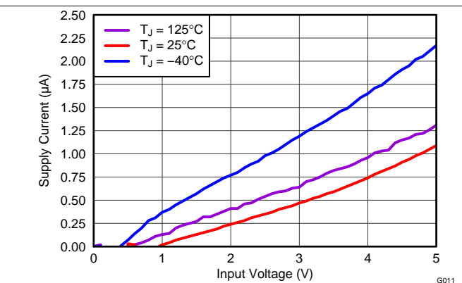
Figure 14. Supply Current (VIN pin) vs Input Voltage (0V to VSTART) EN Pin Low
