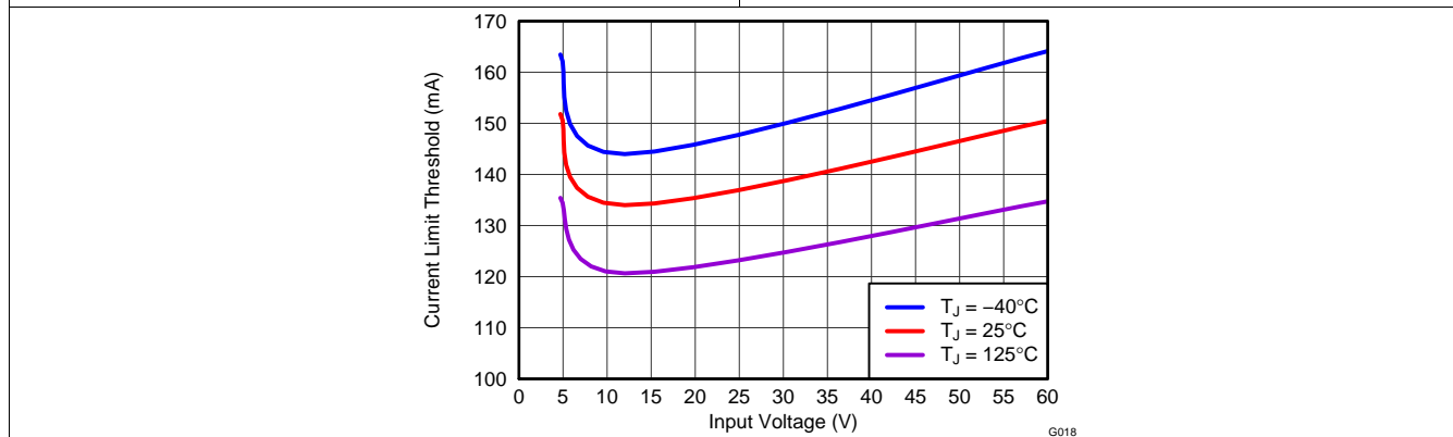
Figure 17. Current Limit vs Input Voltage
