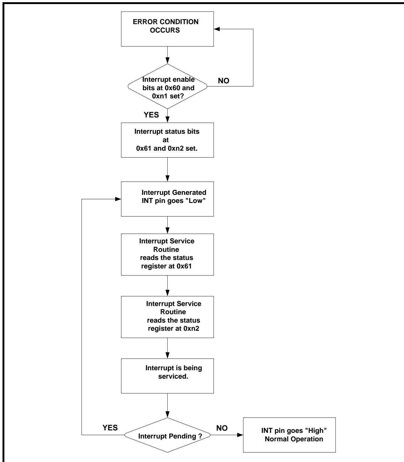
FIGURE 37. INTERRUPT PROCESS
